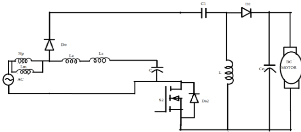
Mode 2 Operation
