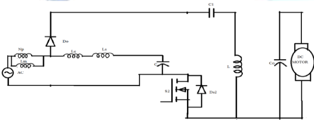
Mode 3 Operation
