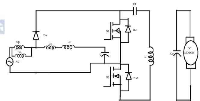
Mode 1 operation
