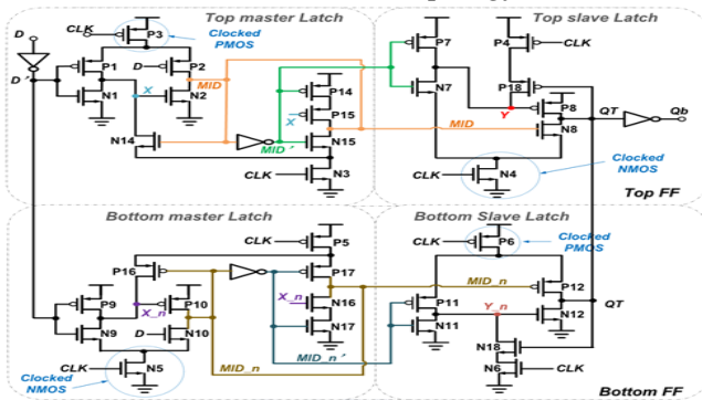
Fig. 4. Proposed TSPC single transistor clocked DET, STC-DET.
