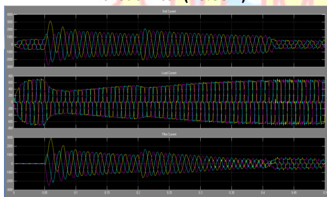
Fig 13 Grid, Load, Filter Current waveforms (Filter on from 0.05 to 0.4)
