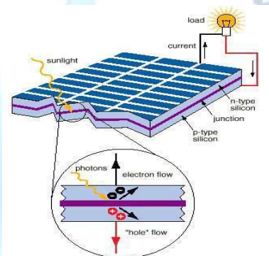
Figure 2 Basic Structure of PV Cell
