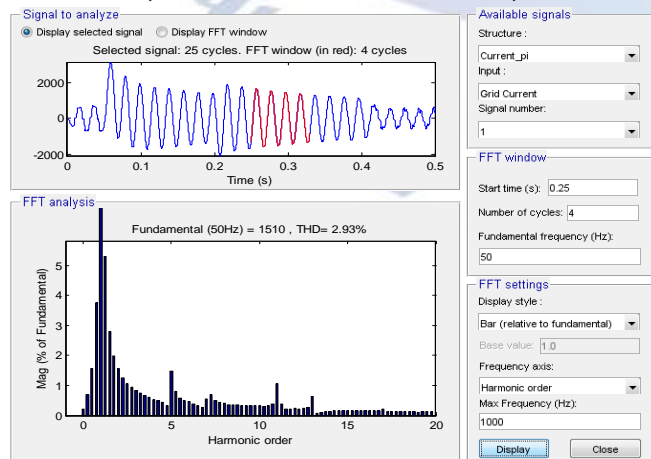
Fig 14 Conventional Circuit THD analysis with filter (2.93%)
