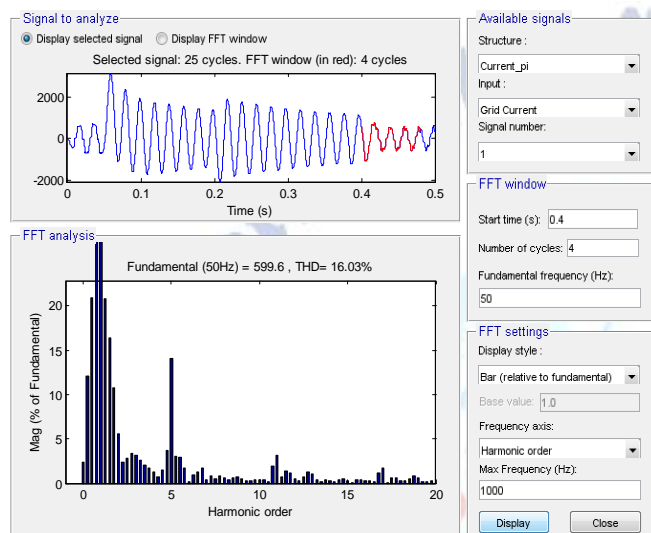
Fig 12 Conventional Circuit THD analysis without filter (16.03%)
