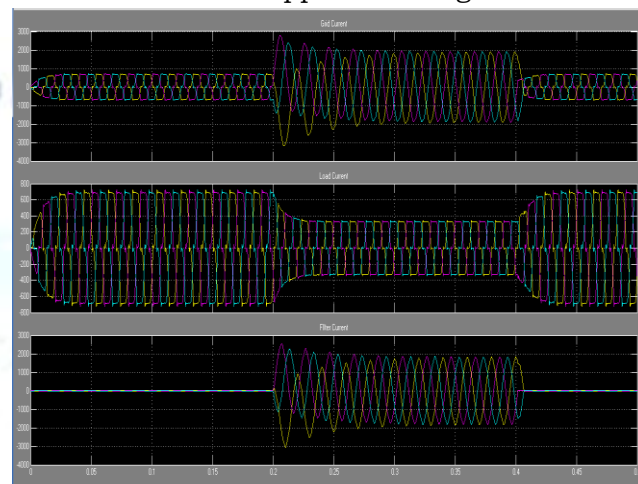
Fig 15 Proposed Method Grid, Load, Filter Current waveforms (Filter on from 0.2 to 0.4)
