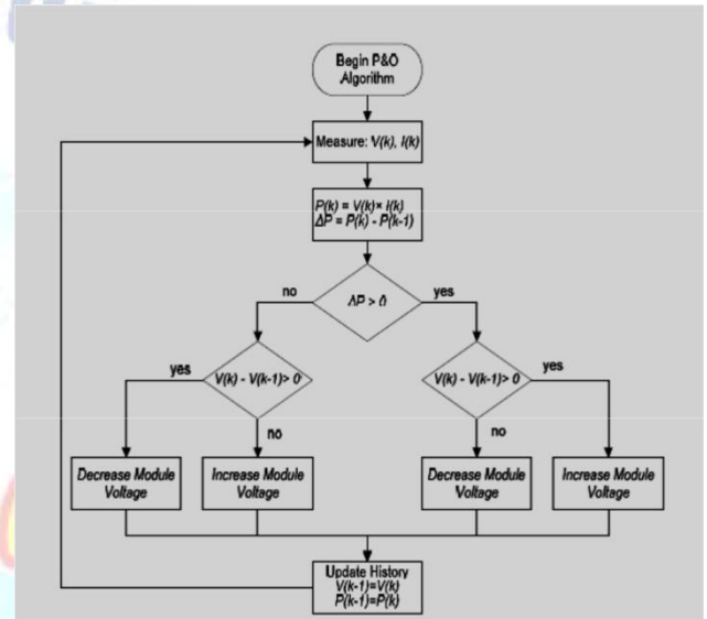
Figure 6 The flow chart of the P&O algorithm
