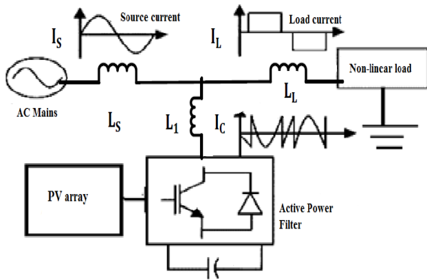
Fig.1 Schematic diagram of active power filter The AC supply is fed the static load , in this case it is the diode based rectifier with resistive and inductive load,
