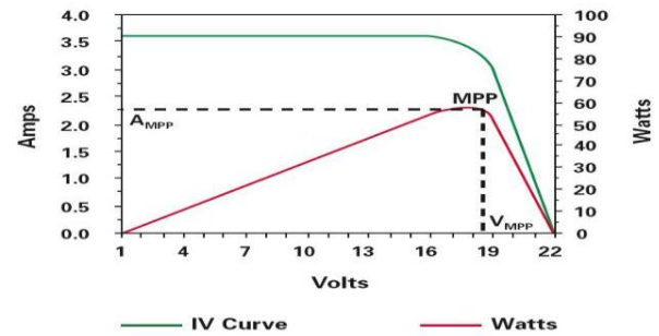
Figure 4 I-V and PV curves
