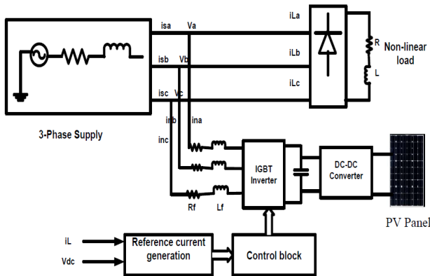
Fig.7 PV system connected to a Shunt APF
