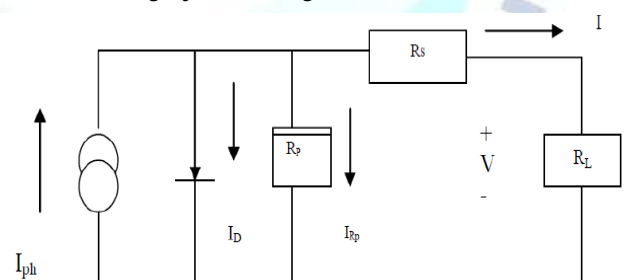
Figure 3 Equivalent circuit of a PV cell
