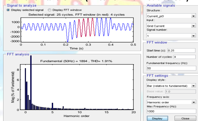
Fig 16 Proposed Circuit THD analysis with filter (1.91%)
