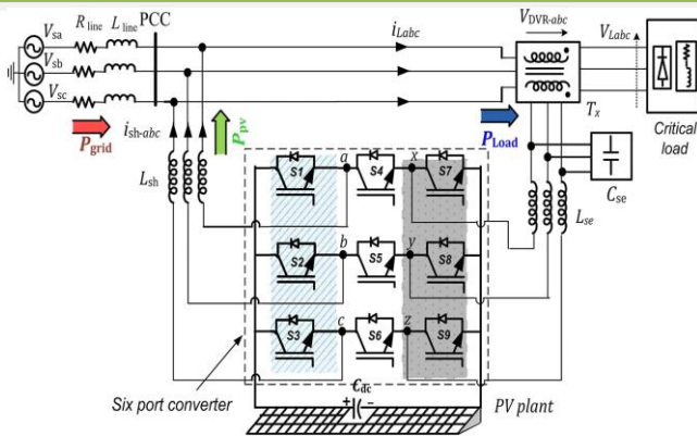
Fig 1: Proposed Configuration of PV with DVR.
