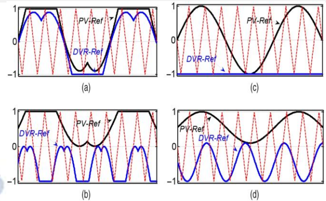
Fig.6: Per phase representation of PV and DVR-VSI modulation references during (a) EF operation; (b) VF operation; (c) healthy grid mode; and (d) sag mode.
