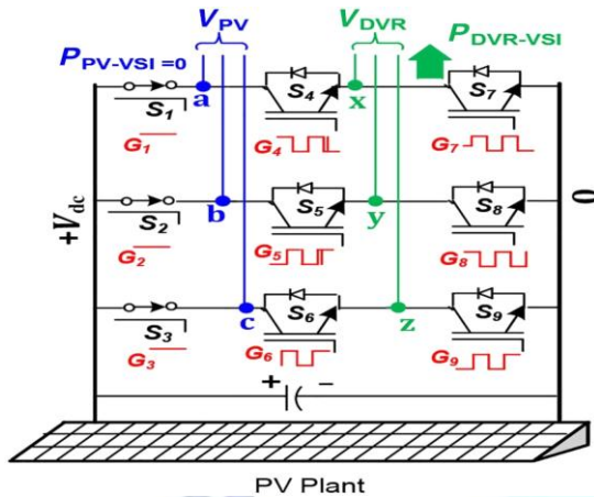
Fig.3: Fault Mode
