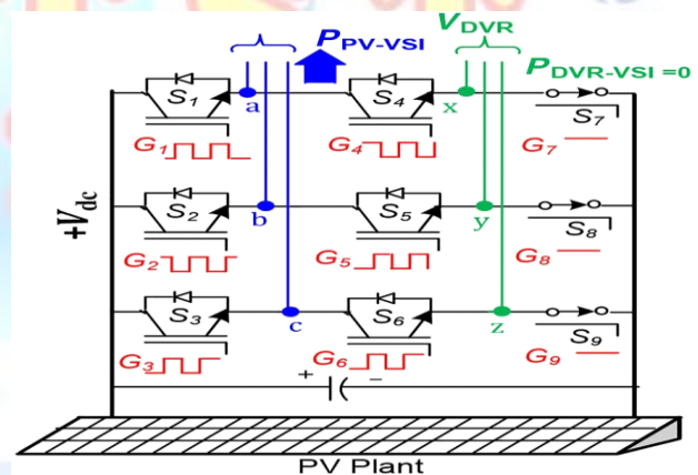
Fig.2: Equivalent Circuit Representation.
