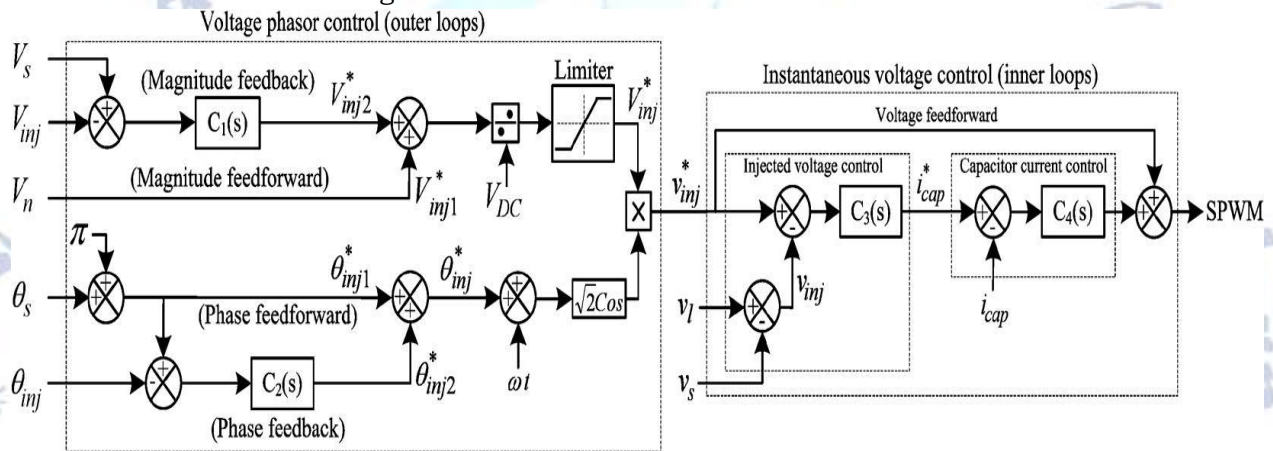
Fig.7: Per-Phase Block Diagram of DVR.
