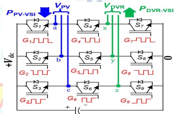
Fig.5: Equivalent System
