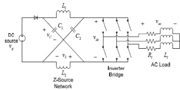
Figure 2.1 ZSC implemented as a three-phase inverter (ZSI)
