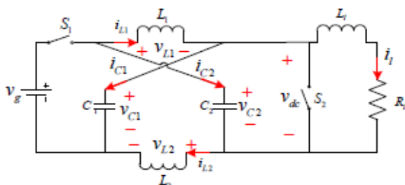
Figure 2.3 Simplified ZSC
