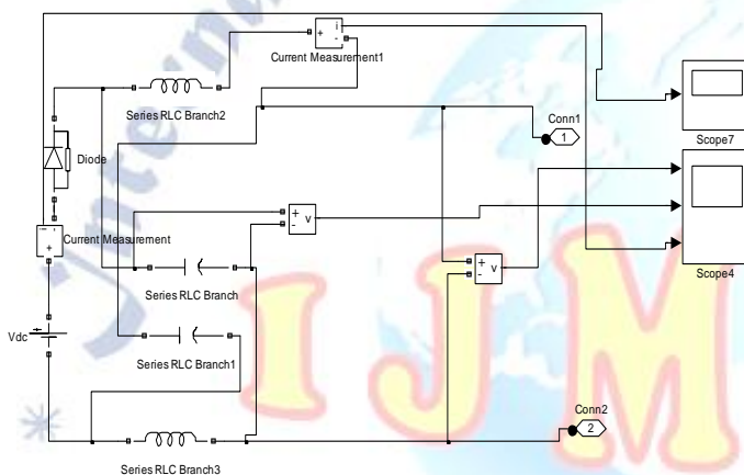
Fig: Simulation circuit of Z-Source
