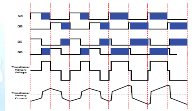
Fig.3 phase shift full bridge circuit
