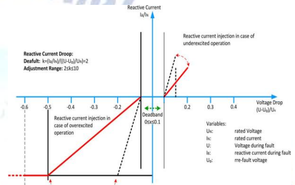
Figure 2.1 REE voltage support requirement in the event of grid fault
