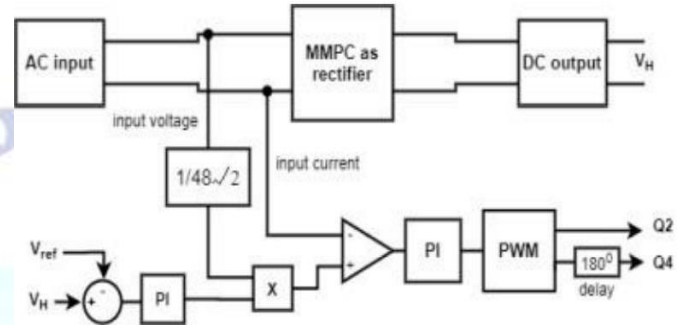
Figure 4: Average current mode control for PFC
