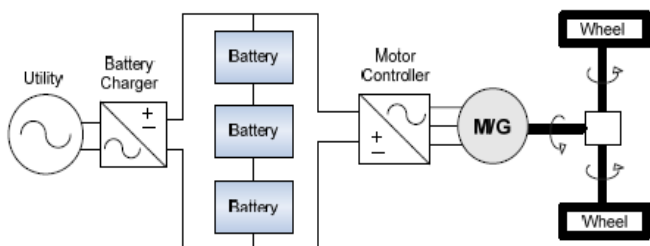
Figure 1: Typical EV configuration
