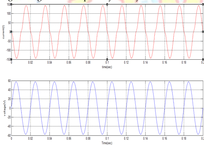
Figure 7: Input Voltage and Current Wave Forms for Ac-Dc Mode
