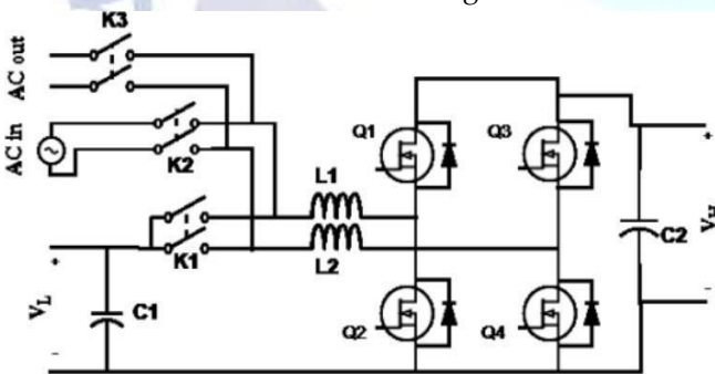
Figure 3: Proposed MMPC Topology
