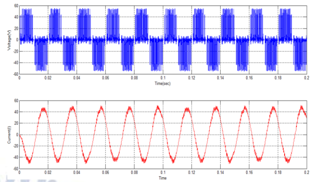
Figure 9: Output Voltage and Current Waveforms for Dc-Ac Mode
