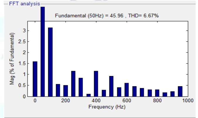
Figure 10: Thd Analysis of Output Current Waveform
