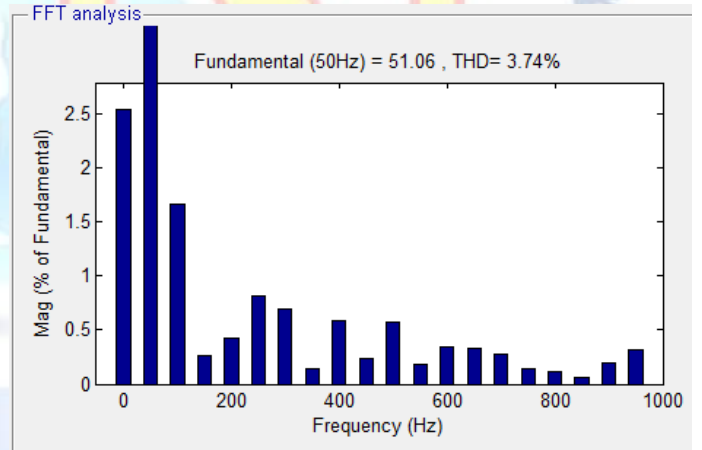
Figure 11: Thd for Output Current in Ac-Dc Mode
