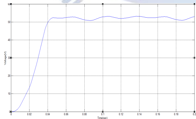
Figure 8: Output Voltage Waveform for Ac-Dc Mode
