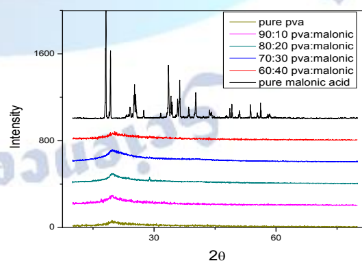
Fig.1a : X-ray diffraction patterns of pure PVA and PVA complexed with Malonic acid
