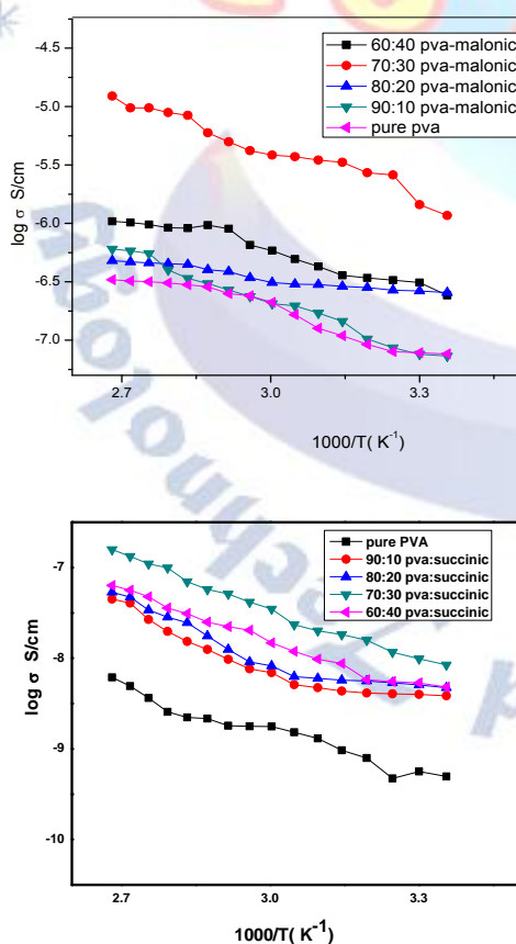
Fig.3: Electrical conductivity as a function of temperature and compositions of PVA-Malonic acid and PVA- Succinic acid.
