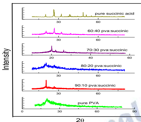
Fig.1b: X-ray diffraction patterns of pure PVA and PVA complexed with succinic acid
