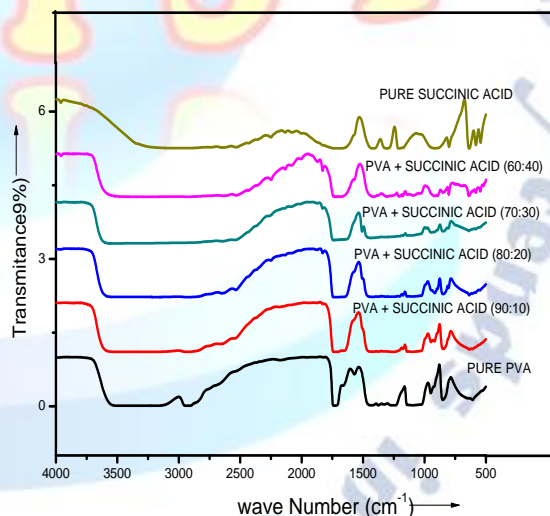
Fig.2b: FTIR spectra of PVA & PVA complexed with Succinic acid polymer electrolytes
