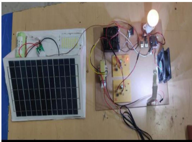
Fig 7. Hardware kit
